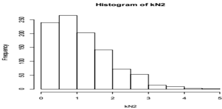
Figure (3.1) the histogram of the sampling distribution of \hat{k}_{HK} , \hat{k}_{N1} and \hat{k}_{N2} when e \sim N(0,1) .
