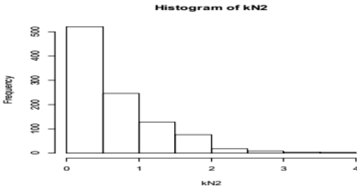
Figure (3.2) the histogram of the sampling distribution of \hat{k}_{HK} , \hat{k}_{N1} and \hat{k}_{N2} when e \sim F(2,10) .
