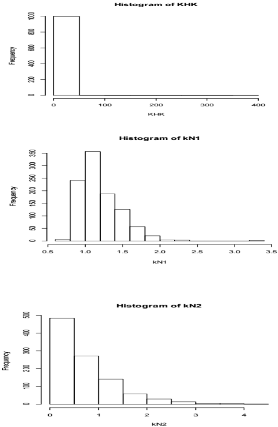
Figure (3.3) the histogram of the sampling distribution of \hat{k}_{HK} , \hat{k}_{N1} and \hat{k}_{N2} when e \sim T_{(4)} .
