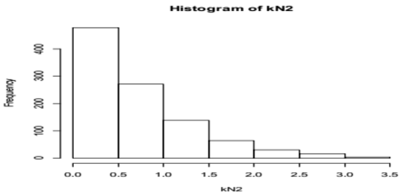
Figure (3.4) the histogram of the sampling distribution of \hat{\mathbf{k}}_{HK} , \hat{\mathbf{k}}_{N1} and \hat{\mathbf{k}}_{N2} when e \sim \chi^2_{(1)} .
